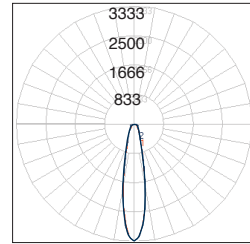
Polar Candela Distribution C6C; 3500K; 12W/ft; 25° x 25°
