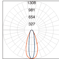
Polar Candela Distribution C6C; 3500K; 9W/ft; 55° x 25°
