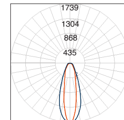
Polar Candela Distribution C6C; 3500K; 12W/ft; 25° x 45°
