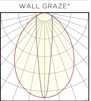
WALL GRAZE* MAX CANDELA: 4185 DELIVERED LUMENS: 4393 WATTS: 32 LPW: 137
