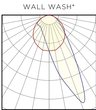
WALL WASH* MAX CANDELA: 3729 DELIVERED LUMENS: 3958 WATTS: 32 LPW: 124
