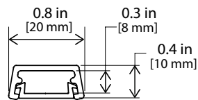
BASE & COVER ASSEMBLY
